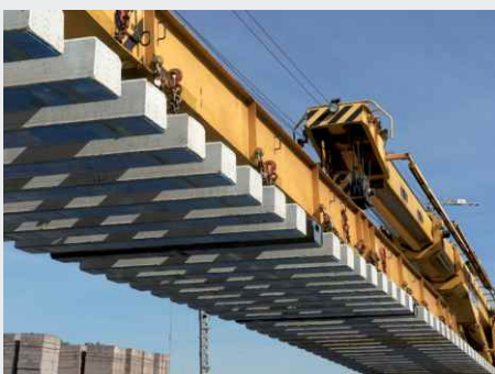
Installation train with switch padding
